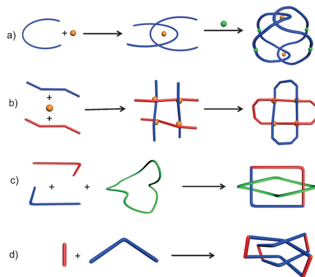
Figure 1. Methods for the synthesis of molecular Solomon links: a) metal templating followed by self-assembly, b) interwoven strategy using metal template followed by ring closing reactions, c) self-assembly using external loop, and d) two-component, coordination-driven self-assembly (this work).
